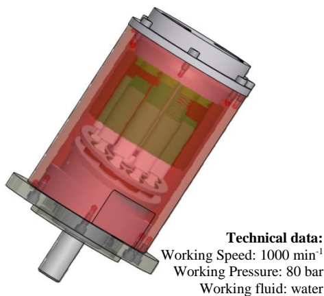
Figure 4. Water hydraulic axial piston pump
