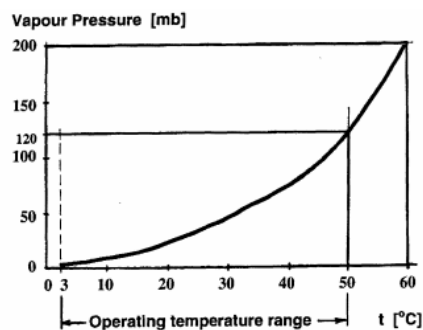
Figure 2. Vapour pressure characteristic of water
