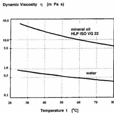
Figure 3. Viscosity of water and mineral hydraulic oil
